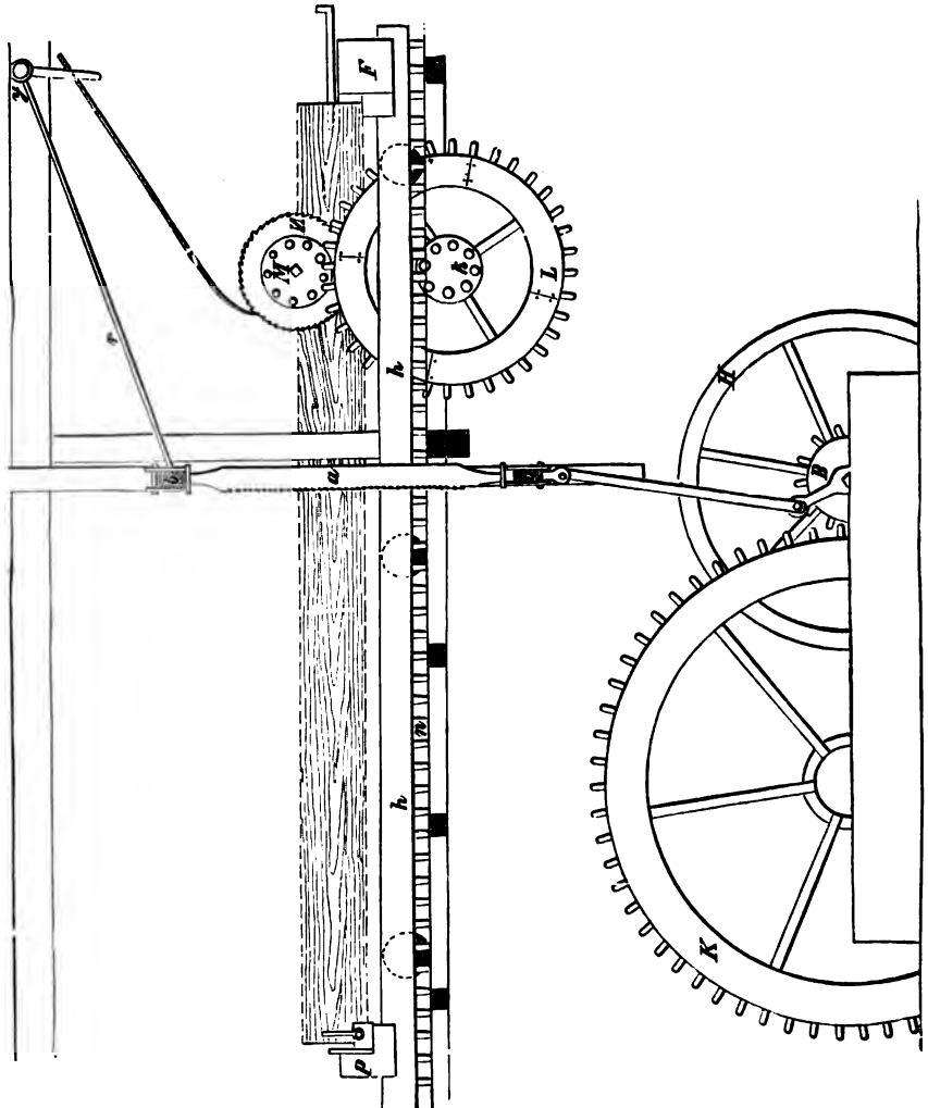
Fig. 297.—Forest sawmill driven by water-power.
